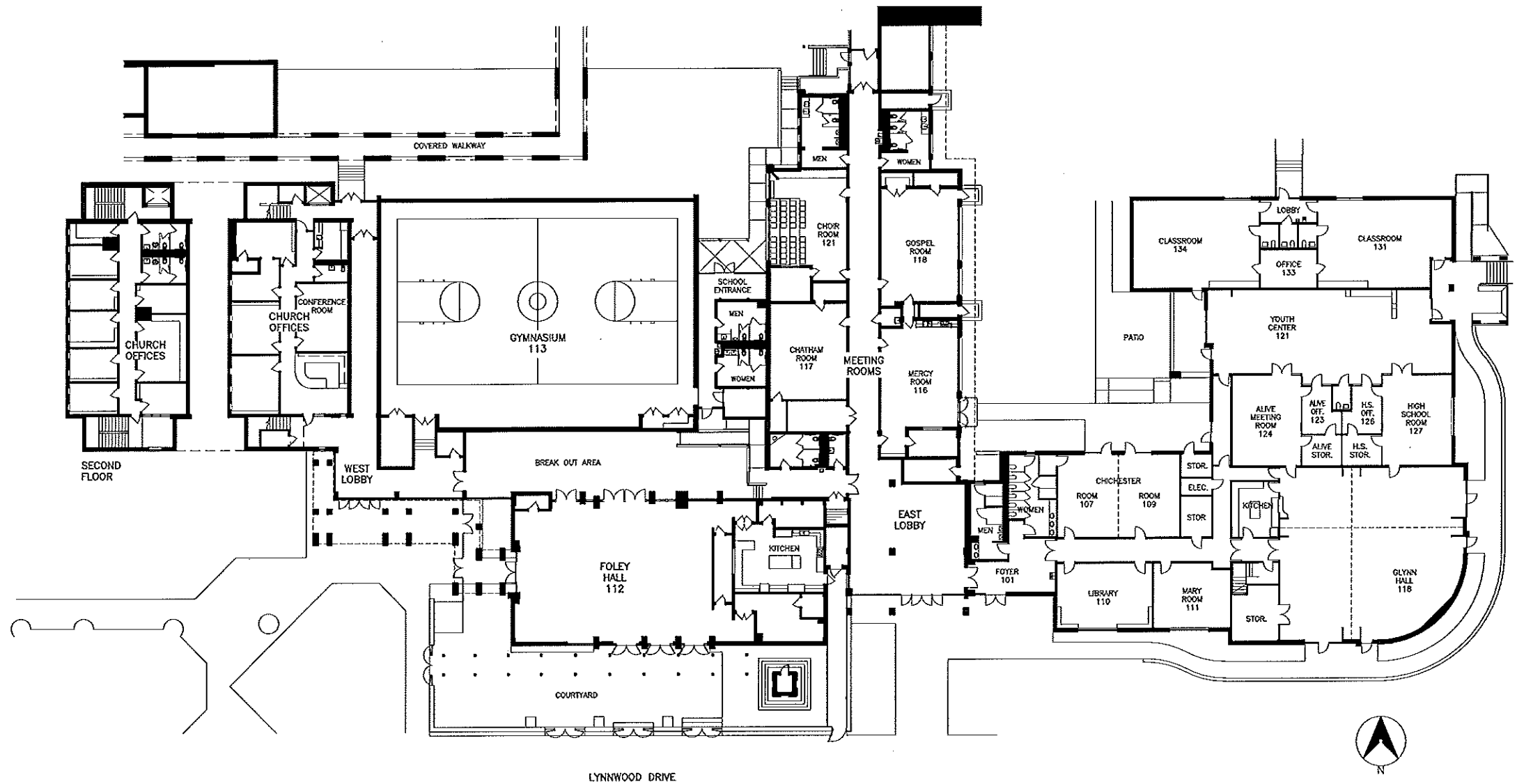
Floor Plan
